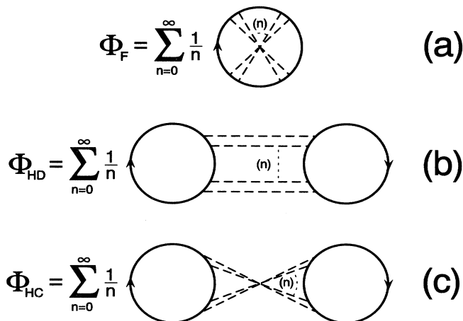
FIG. 3. The generating functional which produces diagrams for (a) weak localization and (b) and (c) the UCF.
